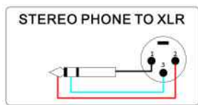
SVP573-10 XLR FEMALE TO TRS JACK (LOCK)
