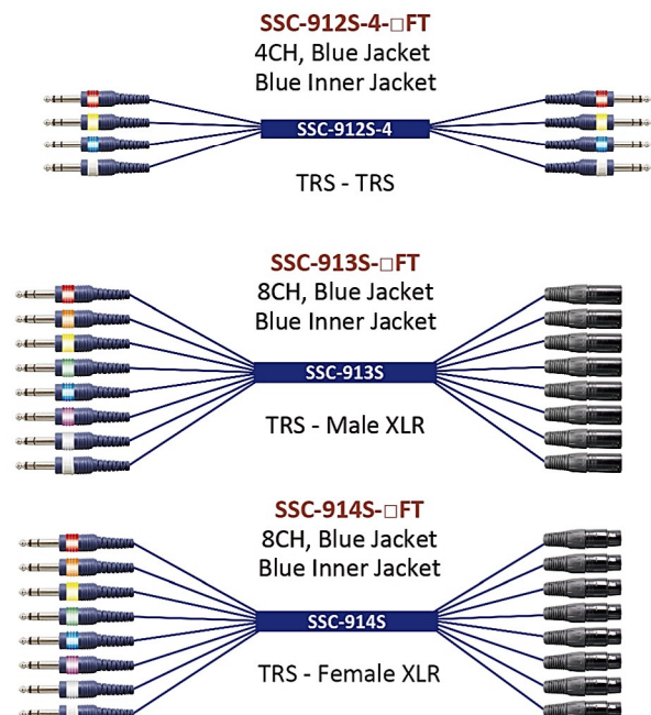
Remark -TB Fantail Stopper, Channel with Heart-shrink PVC Plastic Transparent Tubes and Number Tubes
